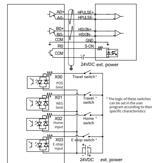
Figure 4 Output terminal wiring
